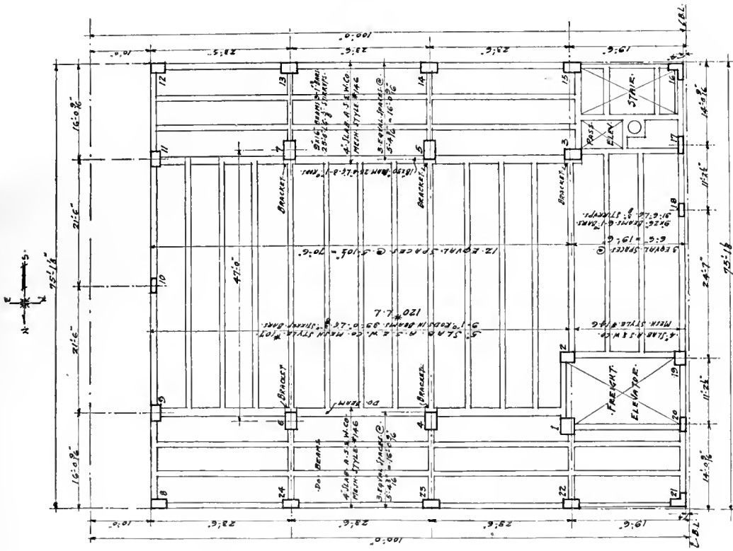
TYPICAL FRAMING PLAN. SCALE: 3/8" = 1'-0"
